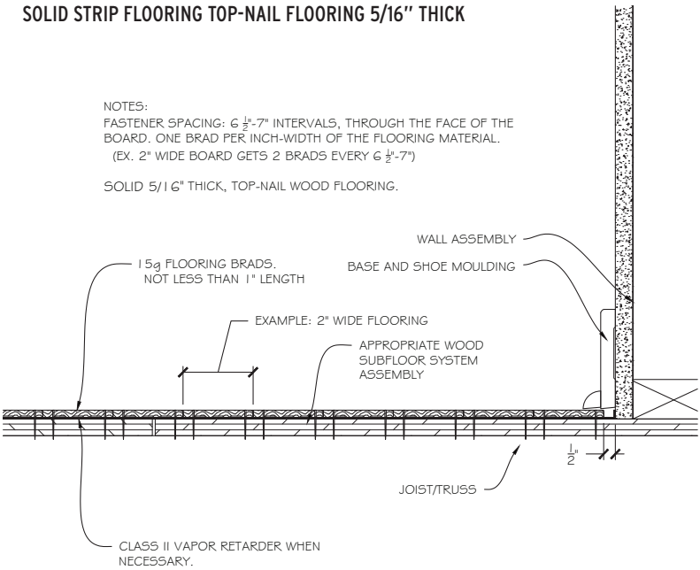
SECTION: WOOD FLOOR INSTALLATION PARALLEL TO FLOOR JOISTS
